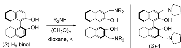
Scheme 2. The general scheme for the synthesis of the amine-containing H 8 -binol ligands such as (S)-1.
